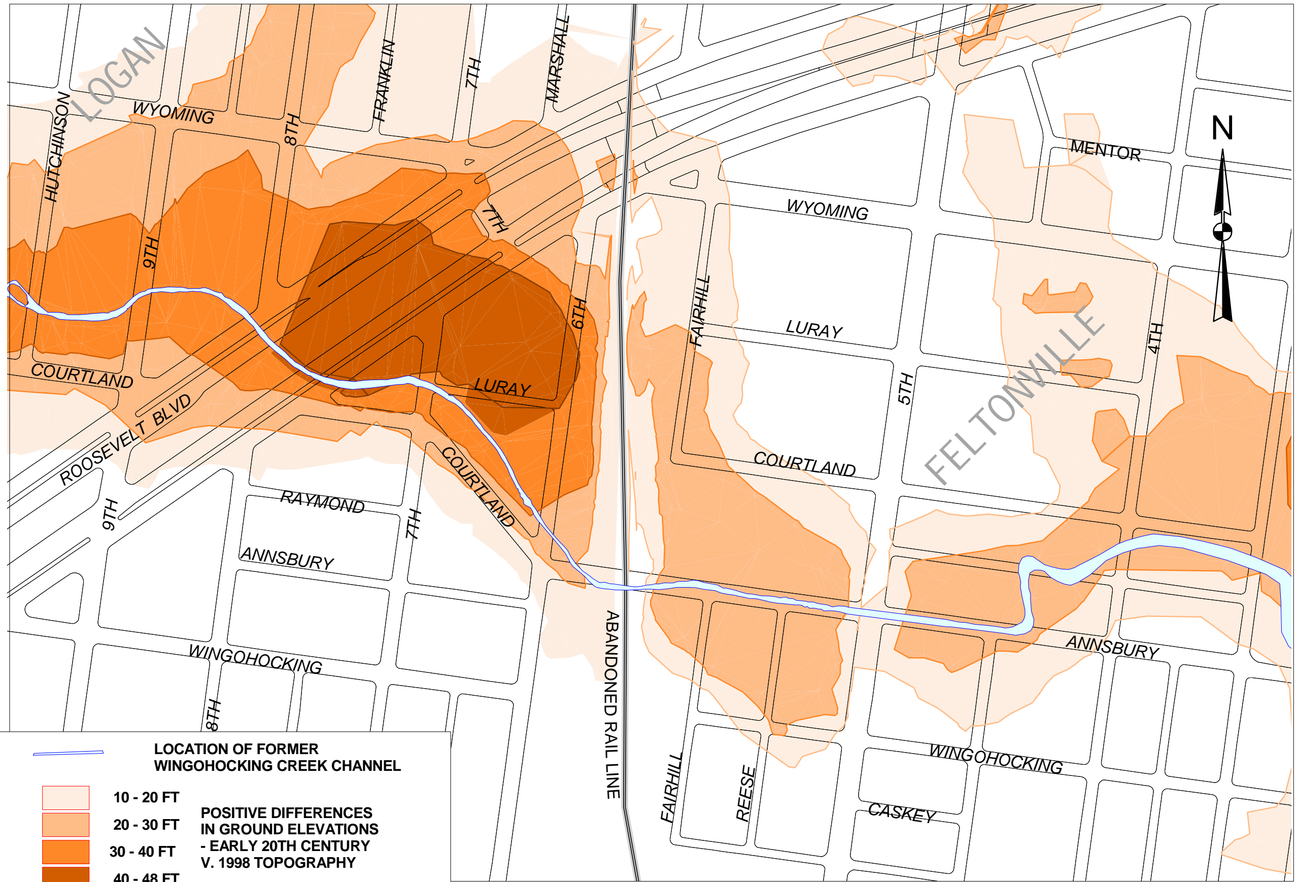
FIGURE FORMER WINGOHOCKING CREEK ESTIMATED DEPTHS OF FILL
